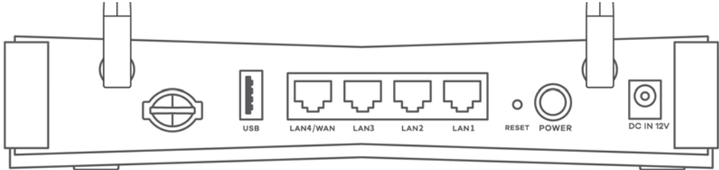
Figure 12 Nebula LTE3301-PLUS
