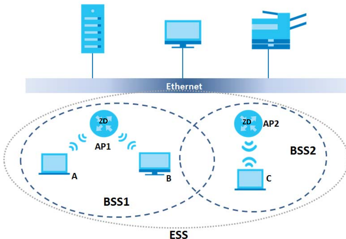
Figure 208 Infrastructure WLAN
